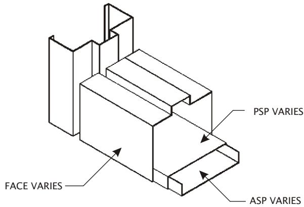
STANDARD BASE PANEL
